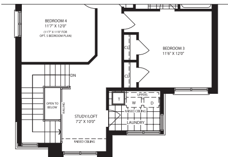
PART: OPT. SECOND FLOOR (5 BEDROOM) ELEV.'B'
